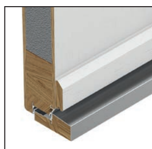
Meleg küszöb Porta ThermControl **
